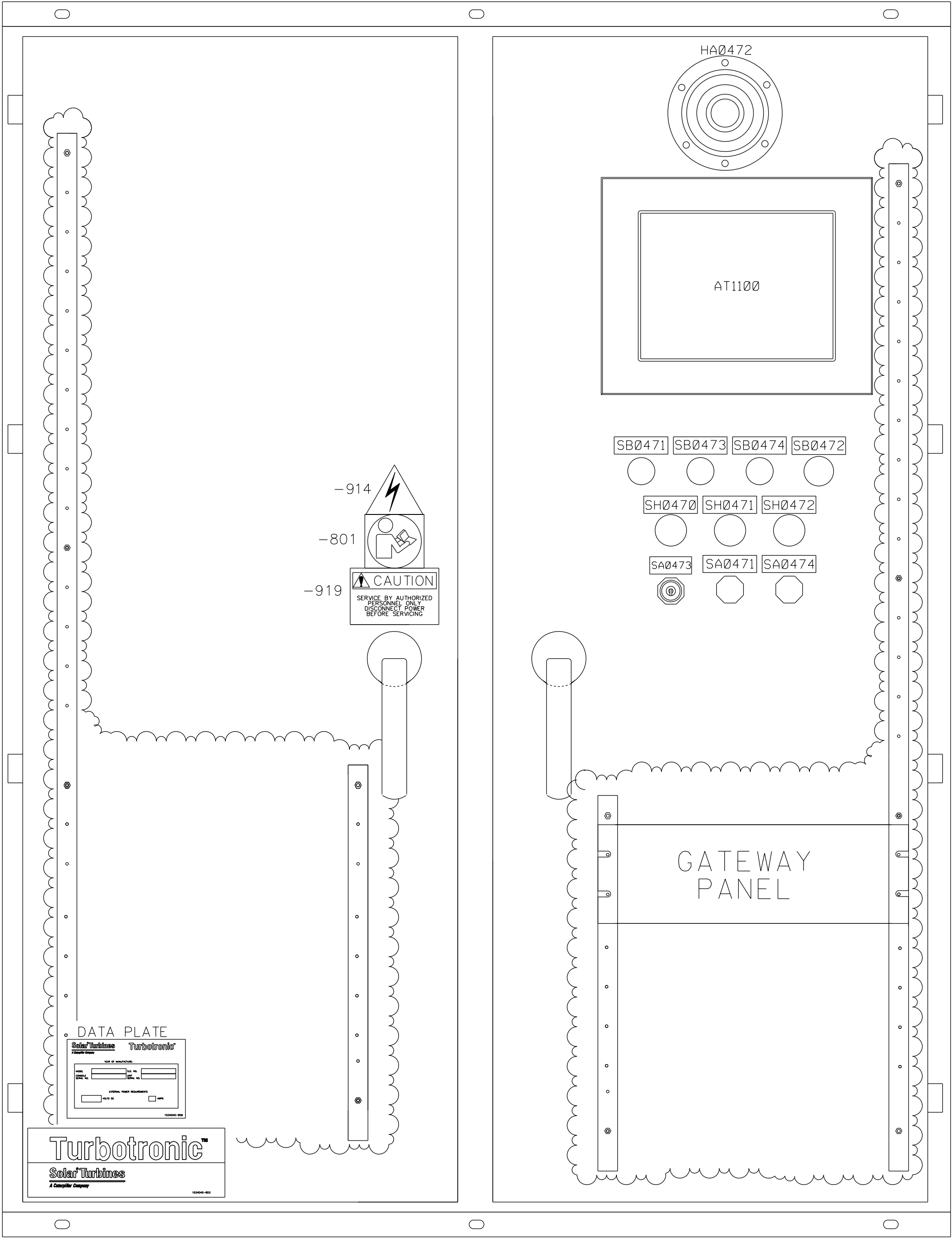
FRONT VIEW
